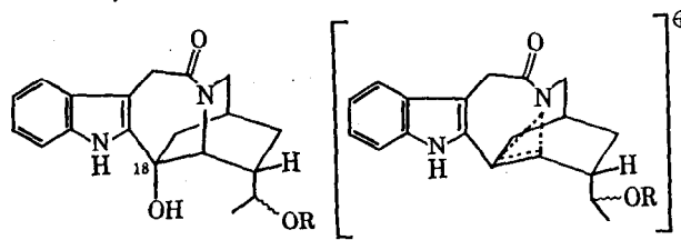
27, R-H 28, R-COCH 3
