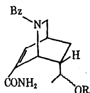
17, R-H 18, R-COCH 3
