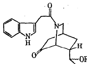
24, R-COCH 3 25, R-H
