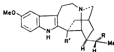
(IIIa) R = H; R' = H Ibogaine (IIIb) R = H; R' = COOMe Voacangine (IIIc) R = OH; R' = COOMe Voacristine
